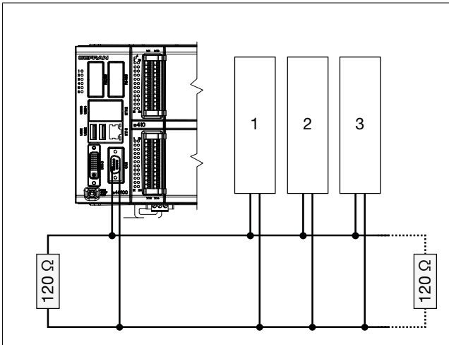
Figure 48 - CAN bus line termination
