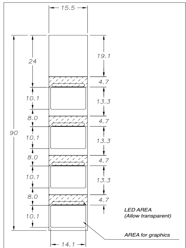
Figure 35 - Label dimensions
