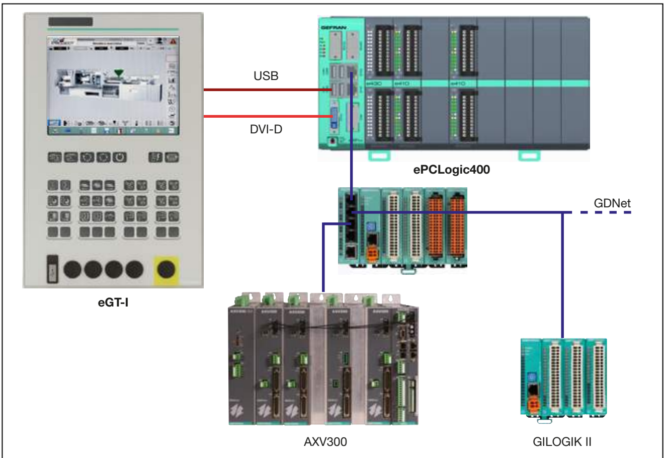
Figure 3 - GDNet System architecture
