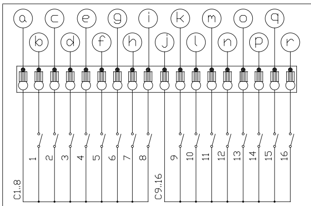
Figure 32 - Diagram of eKM32-104 auxiliary contacts
