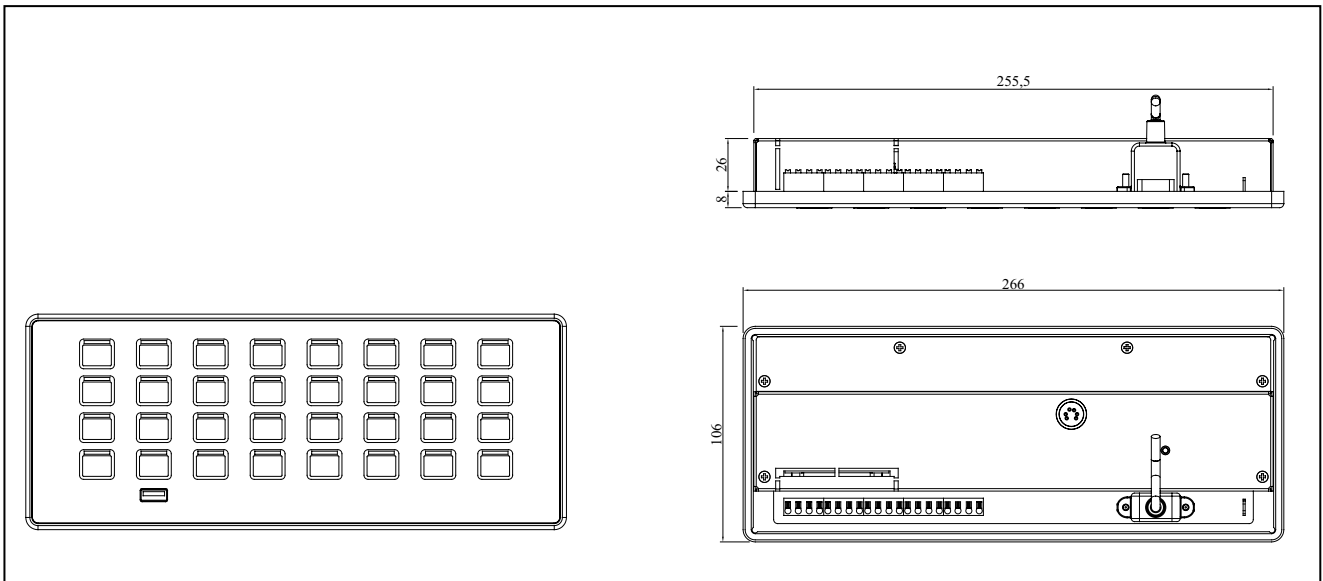
Figure 12 - Dimensions eKM32-104
