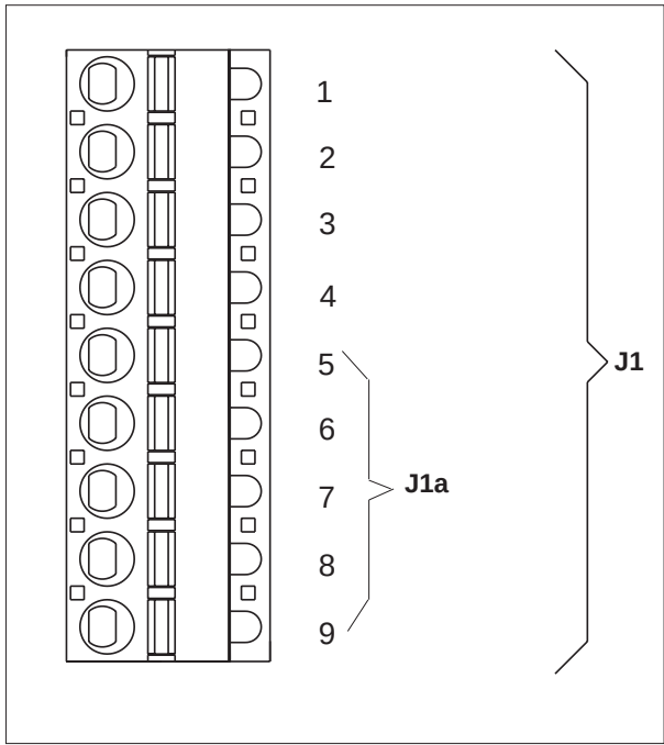
Figure 15 Connector J1
