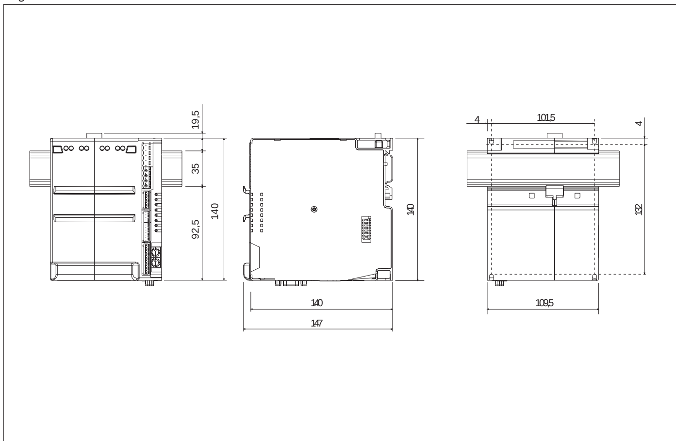
Figure 1 Model without fuse holder
