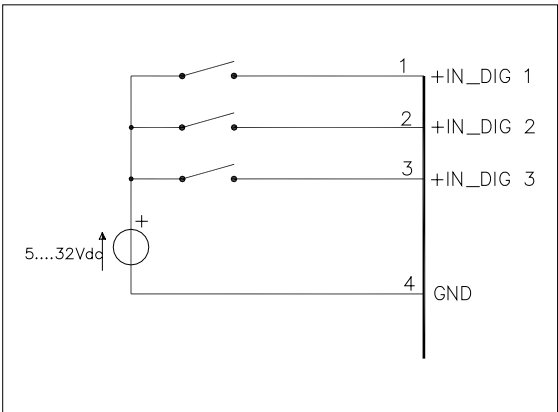
Figure 21 Connection scheme for digital inputs
