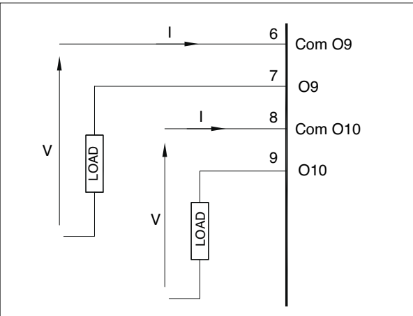
Figure 17 Connection scheme for relay outputs
