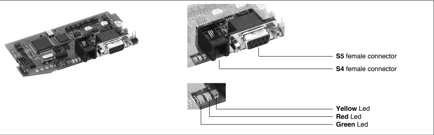
Figure 33 Port2: Fieldbus Modbus RTU/Profibus DP interface
