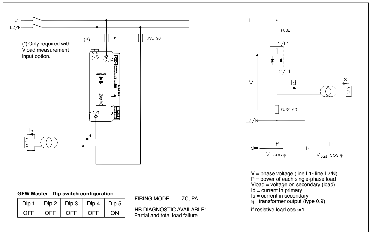
Figura 40 GFW connection example for 1 single-phase transformer load,
