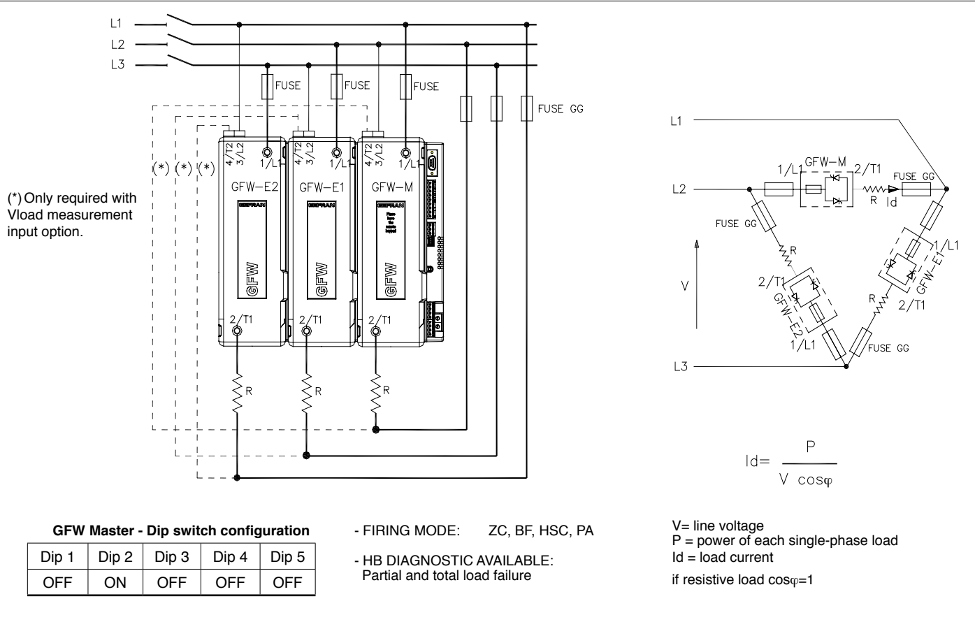
Figure 49 Example of GFW3-PH wiring for 3 independent single-phase loads
