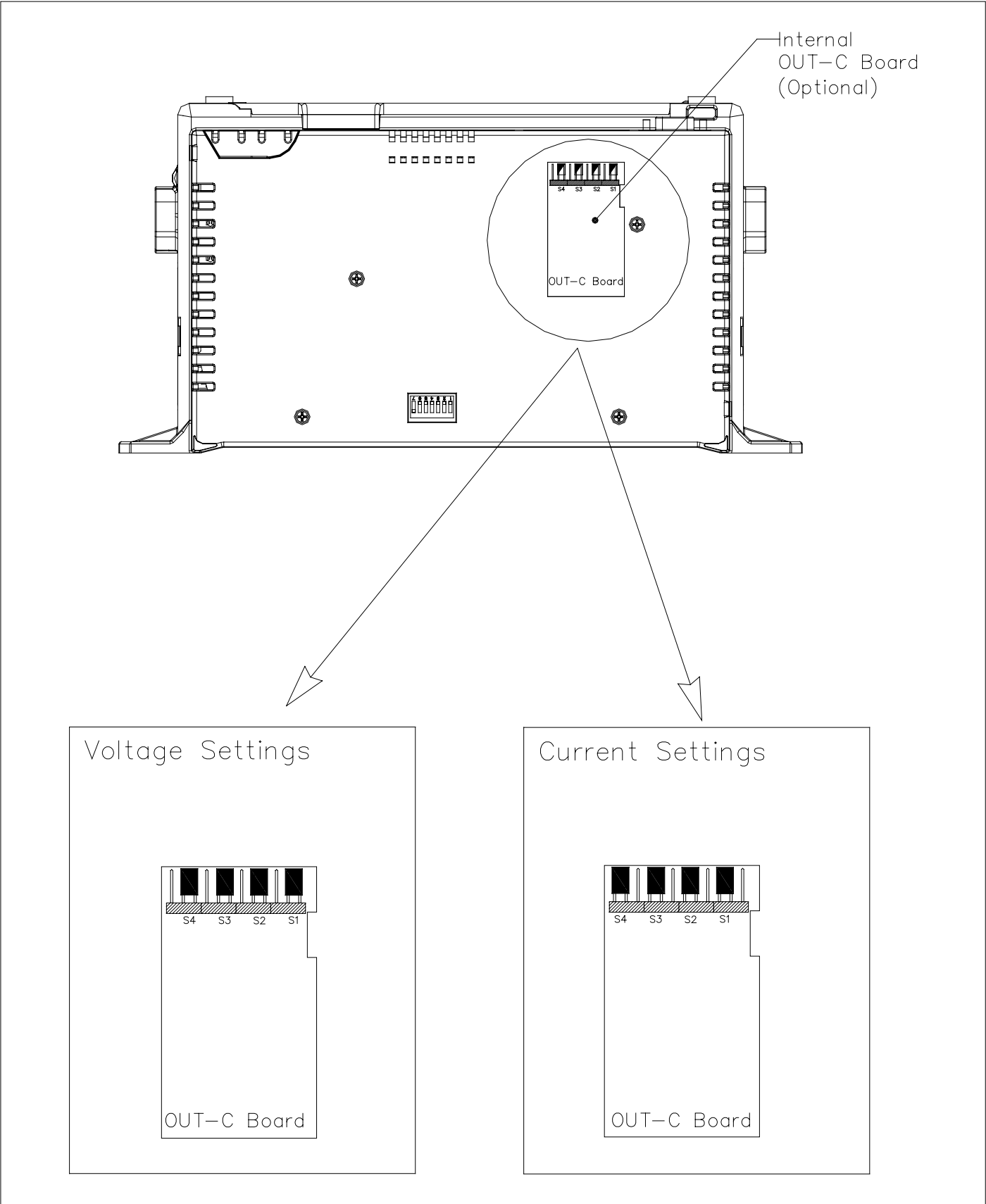
Figure 14 Connection for logic/continuous utputs
