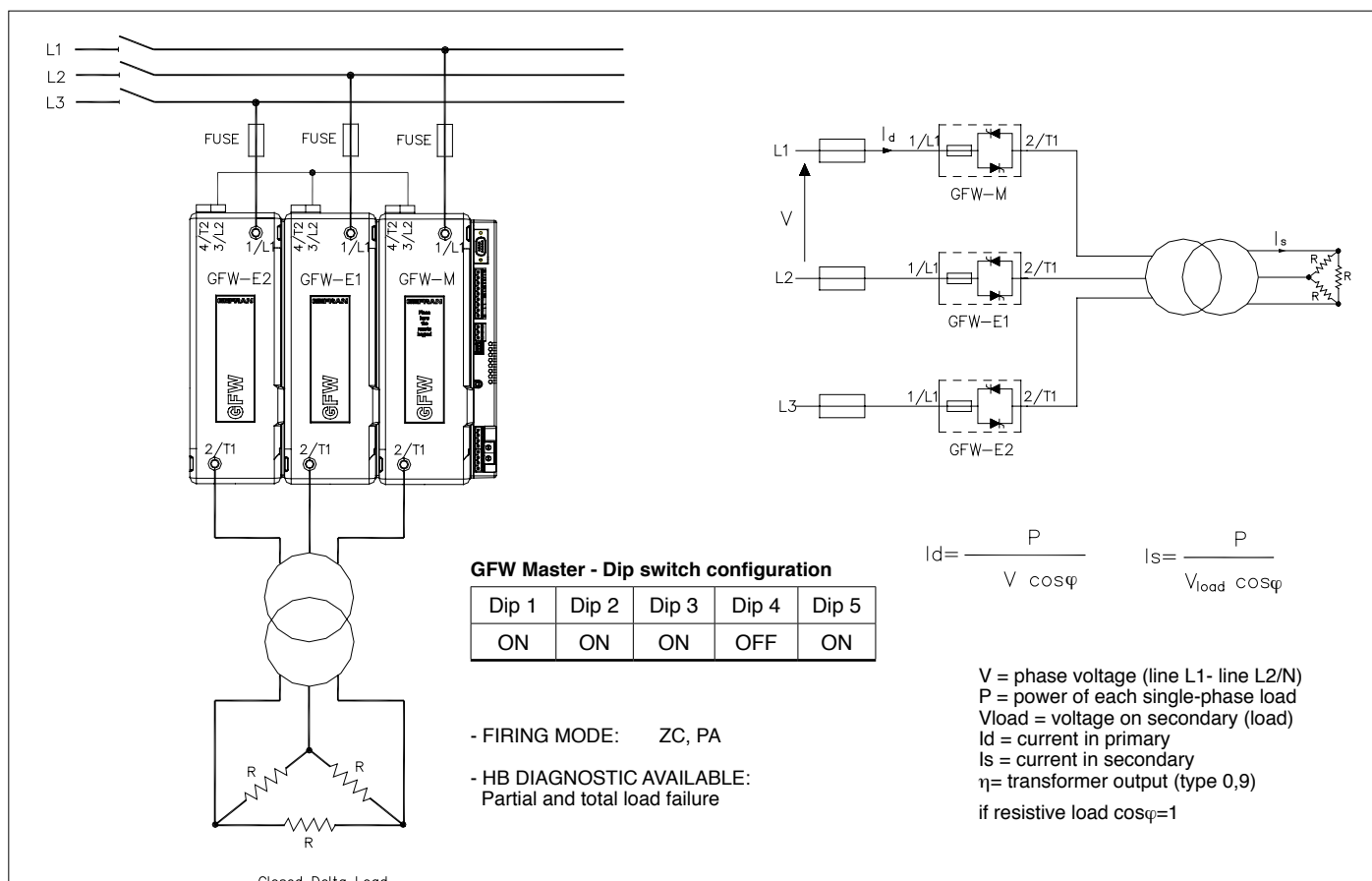
Figura 43 GFW connection example for 1 3-phase closed delta load with transformer
