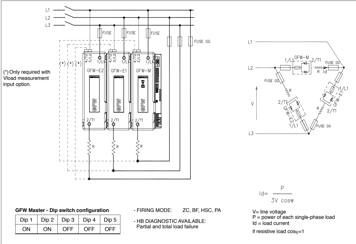
Figure 47 GFW connection example for 1 3-phase load open delta
