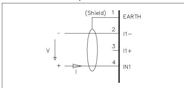
Figure 29 Connection scheme for 1V/20mA linear input
