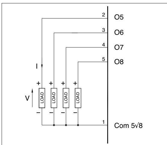
Figure 13 Connection scheme for logic/continuous outputs
