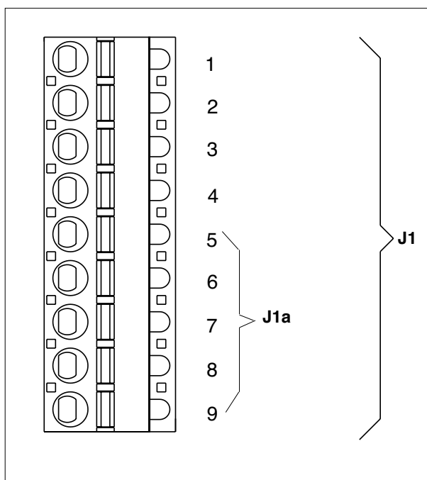
Figure 12 Connector J1
