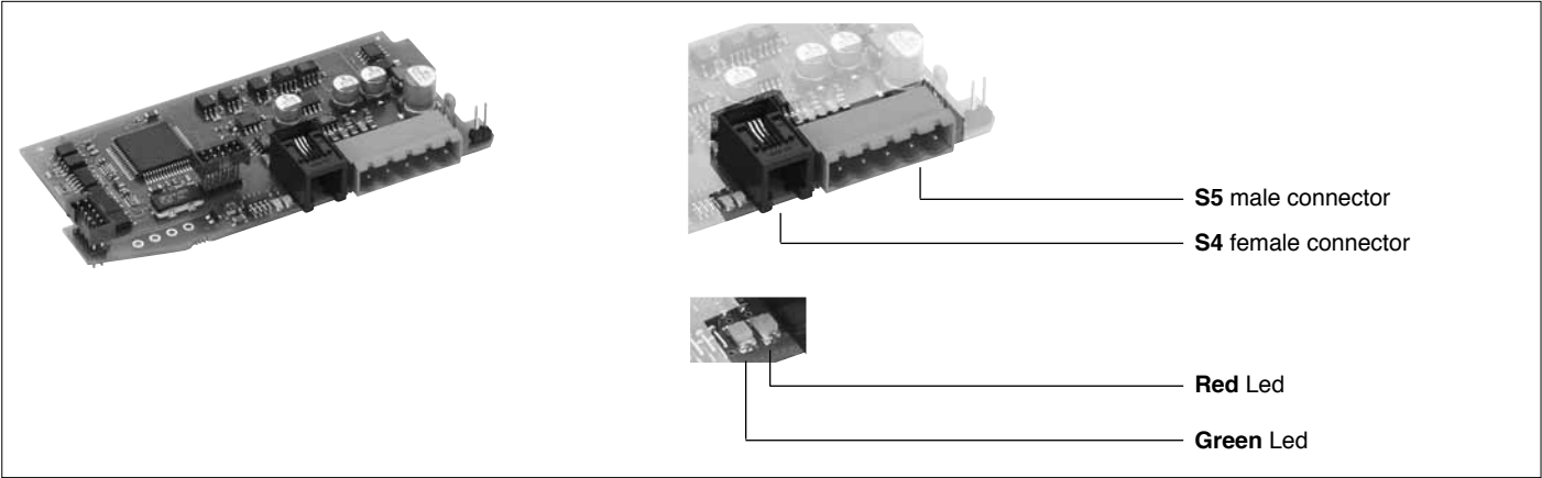
Figure 35 Port2: Fieldbus Modbus RTU/DeviceNet interface
