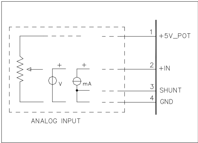
Figure 25 Connection scheme
