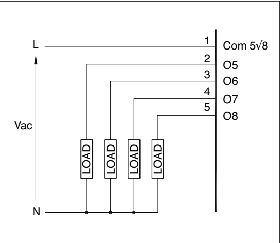
Figure 15 Connection scheme for triac outputs
