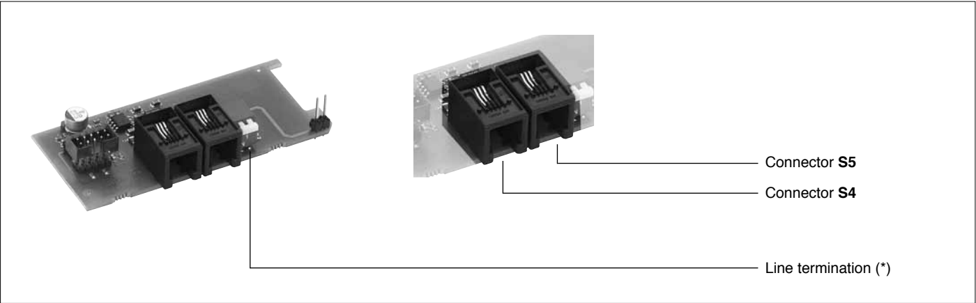
Figure 32 Port2: Fieldbus Modbus RTU/Modbus RTU interface
