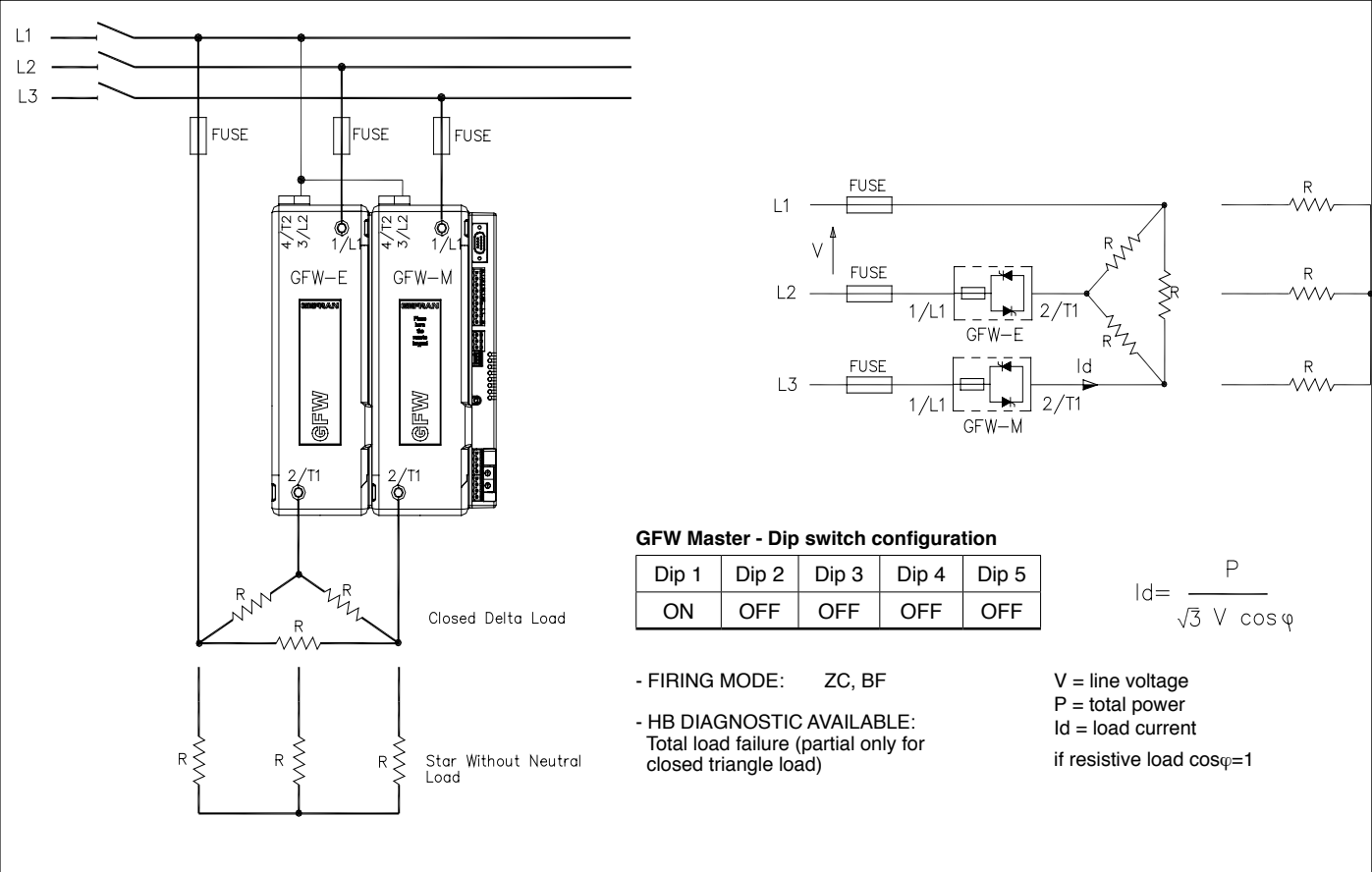
Figure 41 Sample GFW biphas connection for a triphase load
