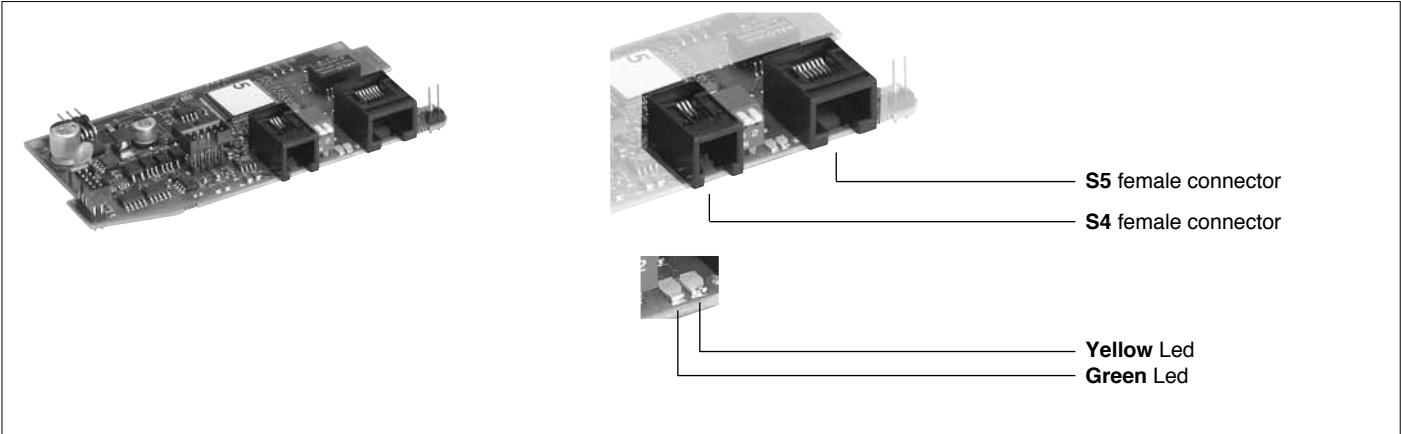
Figure 36 Port2: Modbus RTU / Ethernet Modbus TCP interface
