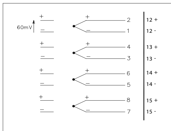
Figure 23 Auxiliary inputs I5 - I8 (60mV/TC)
