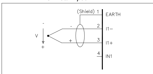
Figure 27 Connection scheme for 60mV TC/linear input
