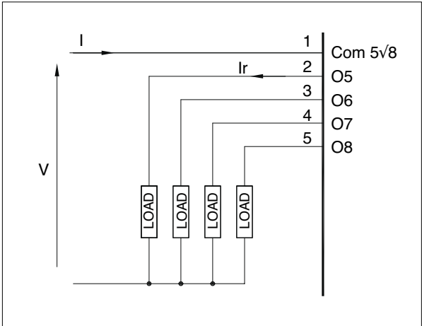
Figure 16 Connection scheme for relay outputs
